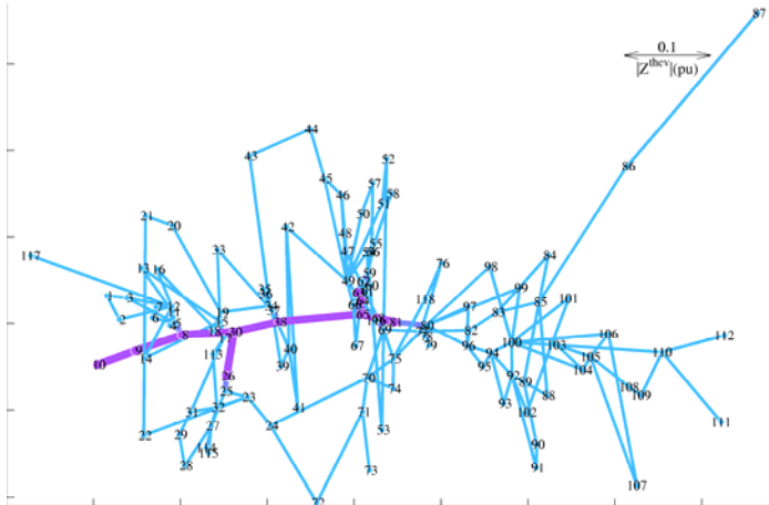
Fig. 3 The IEEE 118 bus system, laid out to show the effective impedance between all node pairs
