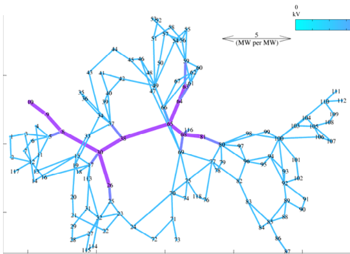
Fig. 1 The IEEE 118 bus system, laid out to show aggregate flow shifts for any node-to-node transaction
