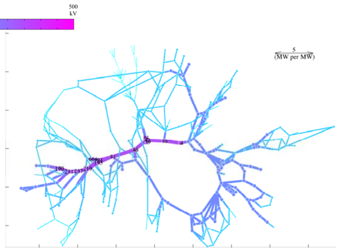
Fig. 2 The IEEE 300 bus system, laid out to show aggregate flow shifts for any node-to-node transaction
